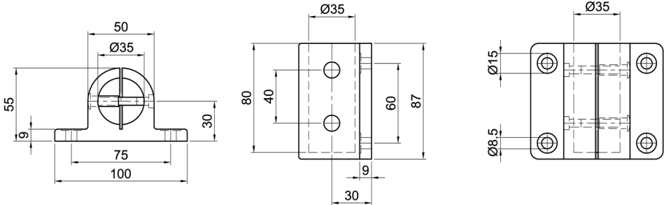
Wandlager, 1-schalig Wall bearing, 1-shell
