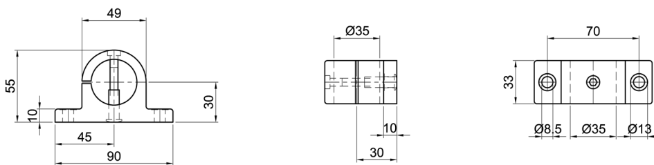
Wandlager, 1-schalig Wall bearing, 1-shell
