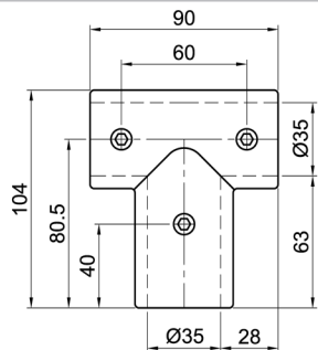
T-Verbinder 45°/135°, 2-schalig T-Connector 45°/135°, 2-shell
