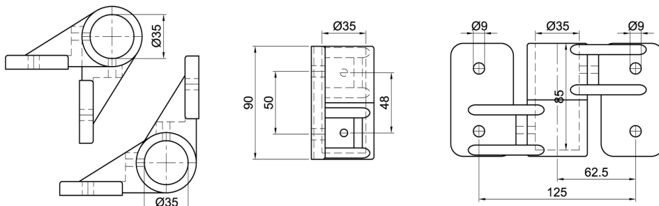
Wandlager-Eckbefestigung, 1-schalig Wall bearing- corner fastening, 1-shell
