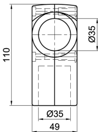
T-Verbinder, 2-schalig T-Connector, 2-shell
